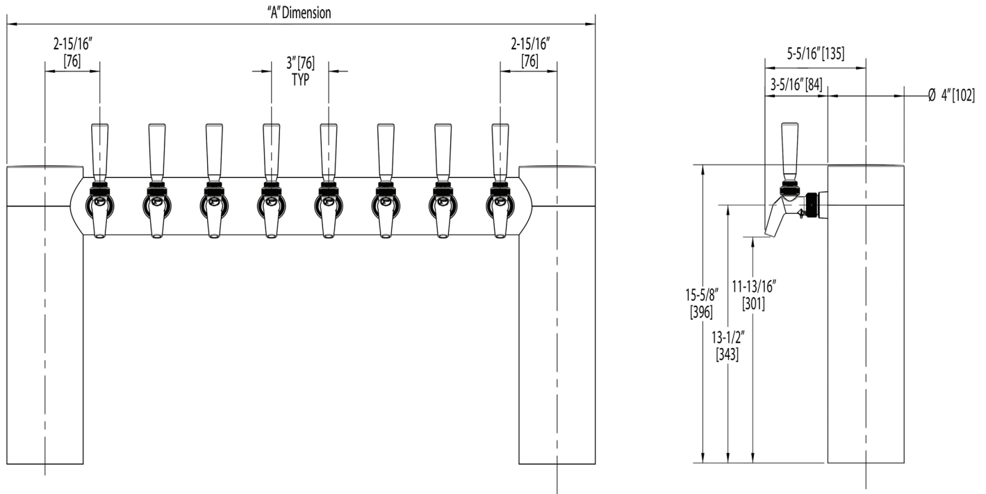
4072-8QC-PO-SS
